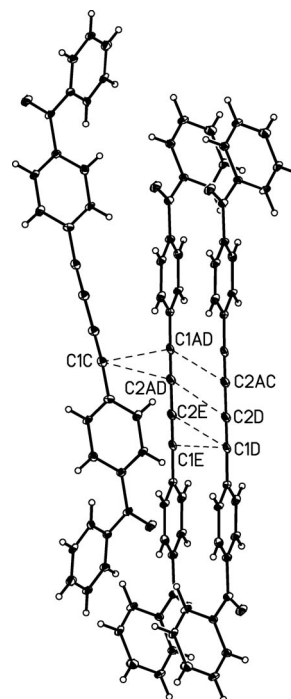
Figure 5. Shortest chain–chain distances for parallel and non-parallel neighbours of 11 . The distances [Å] are: C(1AD)–C(2AC), 3.815; C(2AD)–C(2D), 3.825; C(2E)–C(1D), 3.814; C(1E)–C(1D), 3.902 Å; C(1C)–C(1AD), 4.296; C(1C)–C(2AD), 4.473. Symmetry operations for related atoms are: C(1C): 0.5 - x, 0.5 + y, 0.5 - z ; C(1D) and C(2D): 0.5 - x, 0.5 - y, 1 - z ; C(2AC): x - 0.5, y - 0.5, z ; C(1AD) and C(2AD): x - 0.5, y + 0.5, z ; C(1E) and C(2E): 0.5 - x, 1.5 - y, 1 - z .
