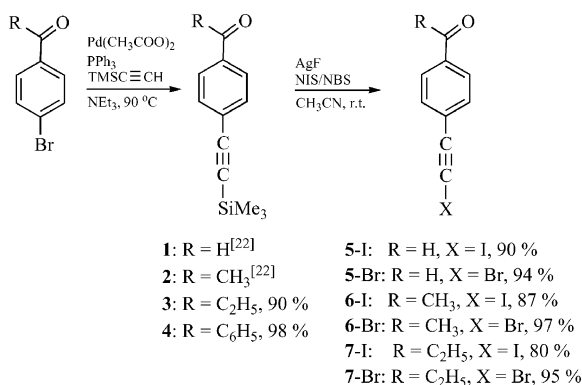
Scheme 1. Synthesis of aryl trimethylsilylacetylenic and haloacetylenic derivatives.
