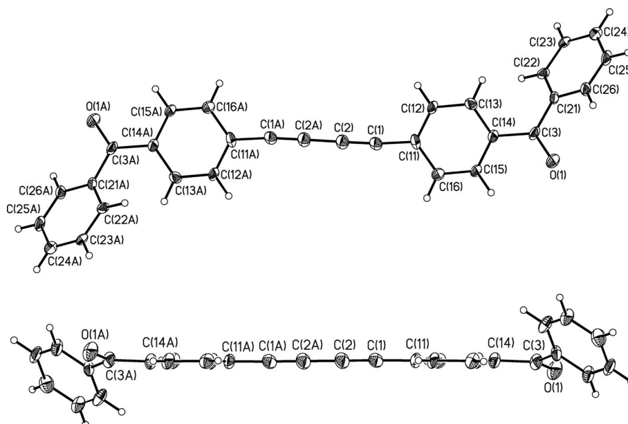
Figure 3. Crystal structure of 11 .
