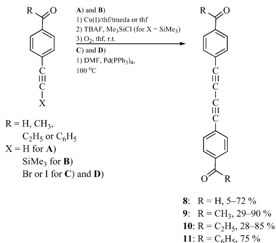
Scheme 2. Synthesis of (keto-aryl)diynes.
