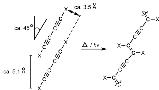
Figure 6. Geometrical conditions for 1,4-topochemical polymerization.
