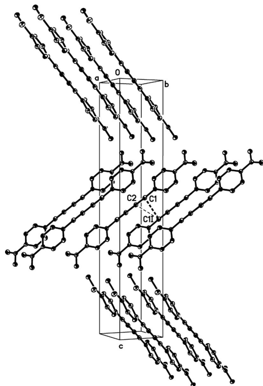
Figure 4. Packing diagram and shortest chain–chain contacts for 9 . The distances are 3.527 Å for C(1)–C(11) and 3.623 Å for C(2)–C(11). Symmetry operation for C(11): 1 - x, 2 - y, 1 - z .
