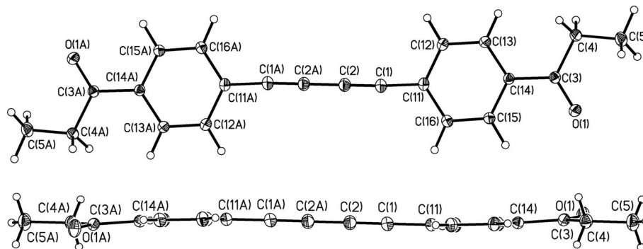
Figure 2. Crystal structure of 10 .
