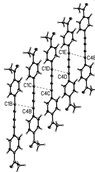
Figure 7. The mutual orientation of molecules of 9 in the crystal lattice. Symmetry operation for related atoms: x, y + 1, z .
